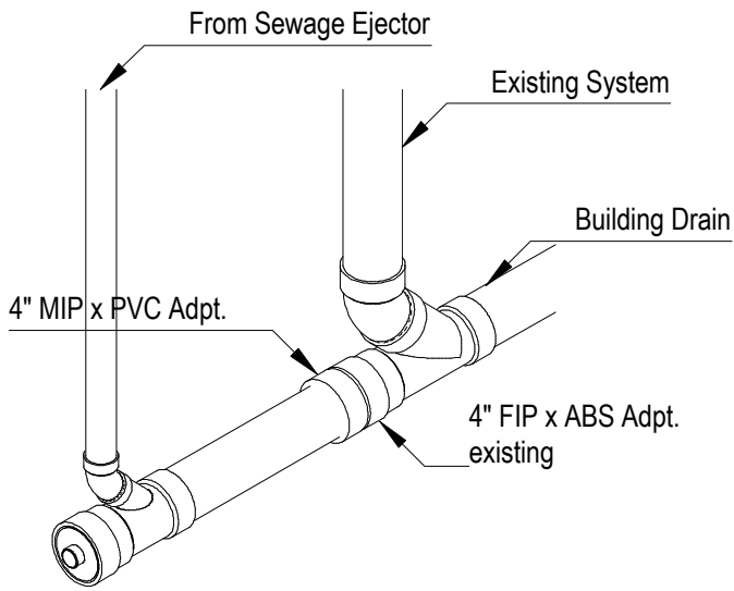
Tie-in Detail
